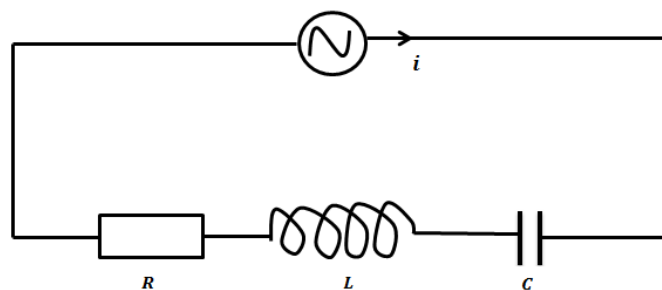
Figure 3. Circuit RLC
